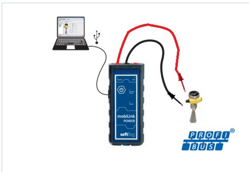
Connection to Profibus PA Device
